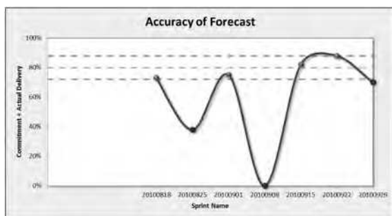
Figure 6. Forecast Accuracy
