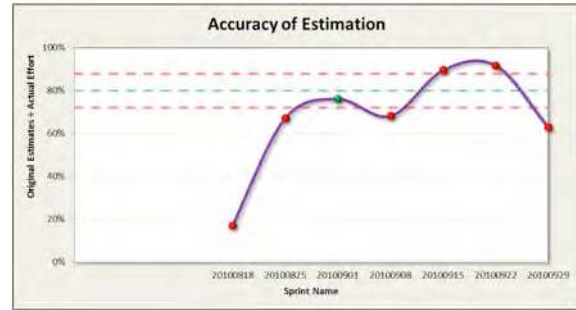
Figure 7. Estimation Accuracy
